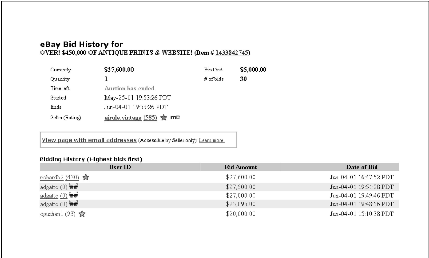
Figure 3. Late Bidding as Best Response to Incremental Bidding.
